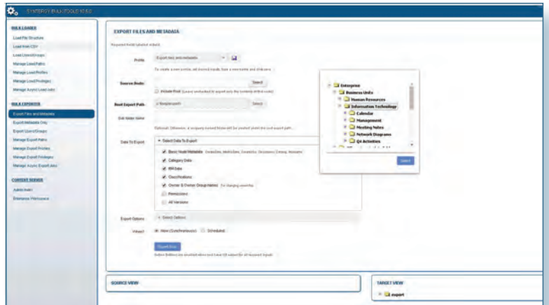
Data Manager Export page: identify and download entire hierarchies from Content Server to your local environment
